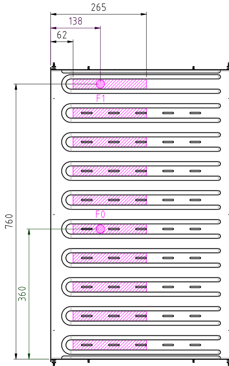
A-A view from inside left
