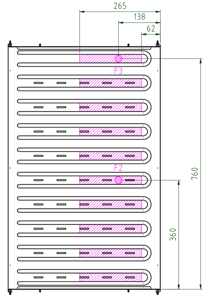
B-B view from inside right
